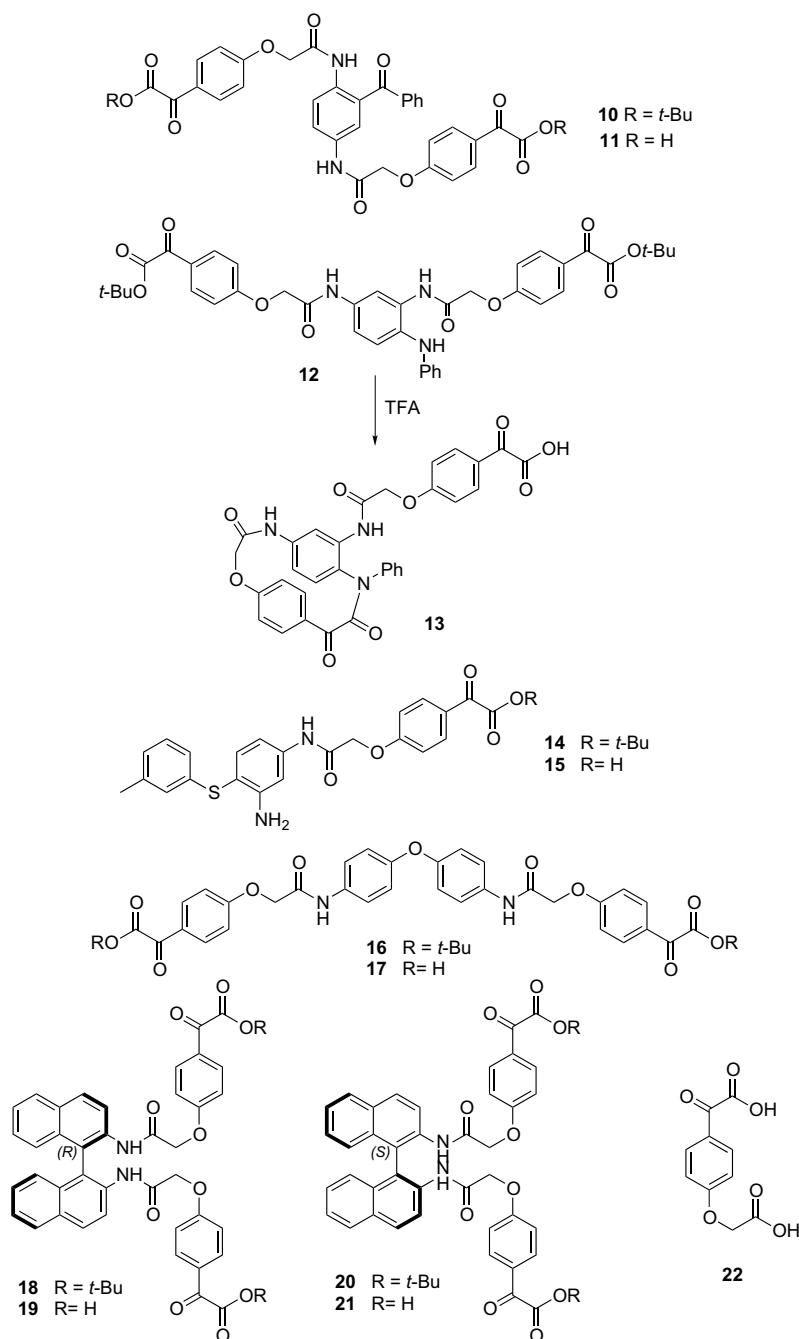
Figure 2. Six best inhibitors, their protected forms and compound 22 ( \alpha -ketoacid form of compound 3 ).
