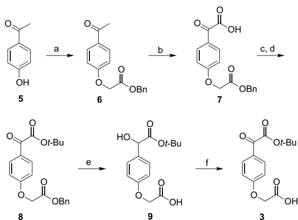
Scheme 2. Reagents: (a) benzyl bromoacetate, K_2CO_3 , DMF; (b) SeO_2 , pyridine, reflux; (c) SOCl_2 , benzene, reflux; (d) t -BuOH, pyridine, CH_2Cl_2 ; (e) H_2 , Pd(OH)_2 , EtOAc; (f) Dess–Martin periodinane, acetone.
